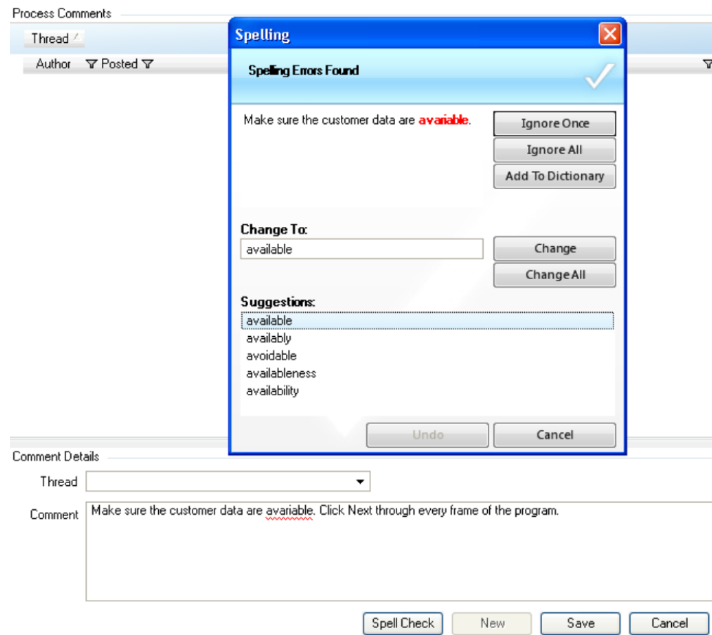
Fig. 2.51 Add Comments
