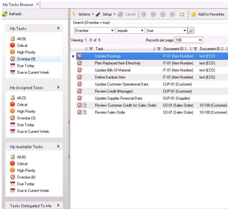
Fig. 2.15 Predefined Filters
