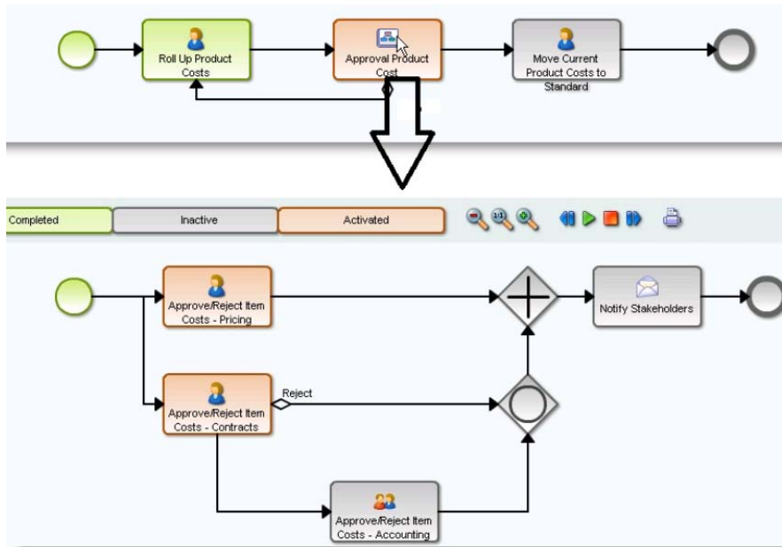
Fig. 2.21 Approval Subprocess
