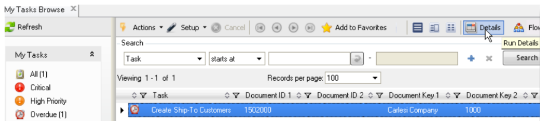
Fig. 2.16 Task Details
