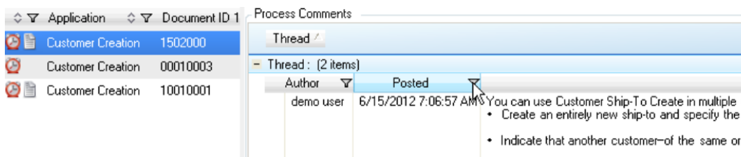
Fig. 2.53 Filter Comments
