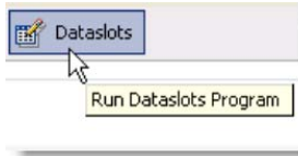
Fig. 2.35 Dataslots button
