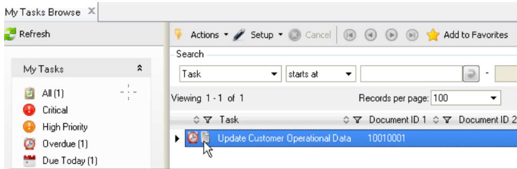
Fig. 2.52 View Comments
