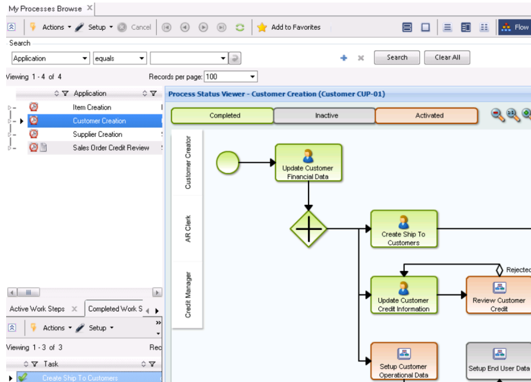
Fig. 2.32 Flow View
