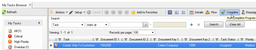
Fig. 2.20 Complete Tasks
