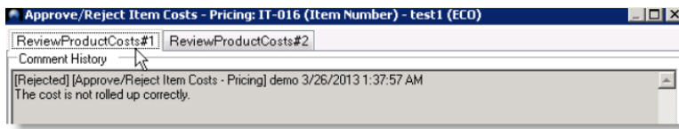
Fig. 2.24 Rejection History
