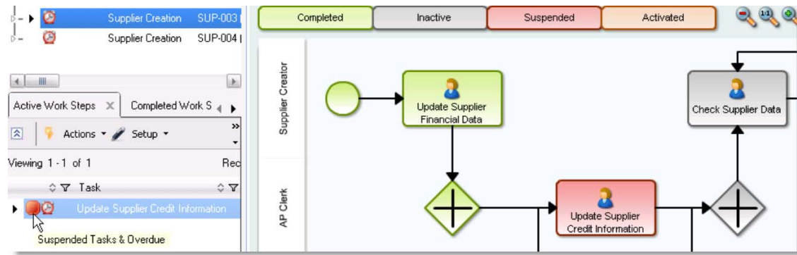
Fig. 2.39 Suspended Task
