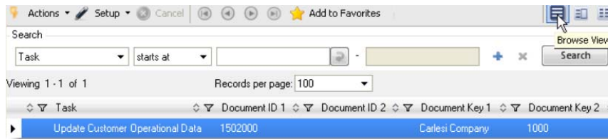
Fig. 2.8 Browse View
