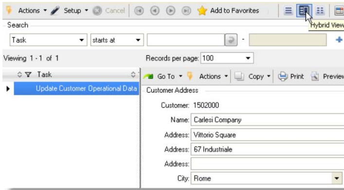
Fig. 2.6 Hybrid View
