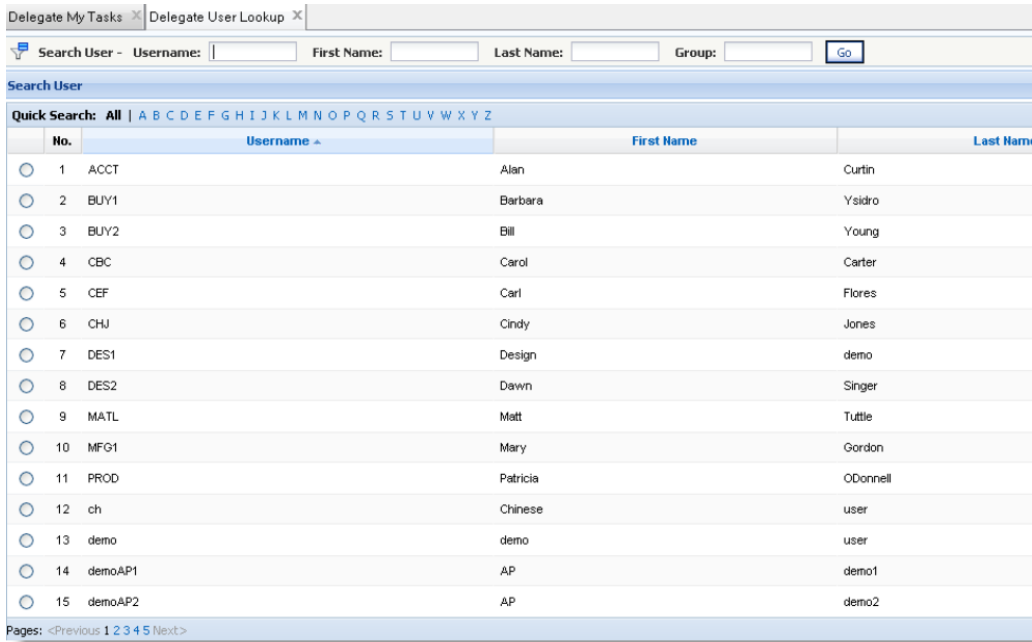
Fig. 2.30 User Lookup
