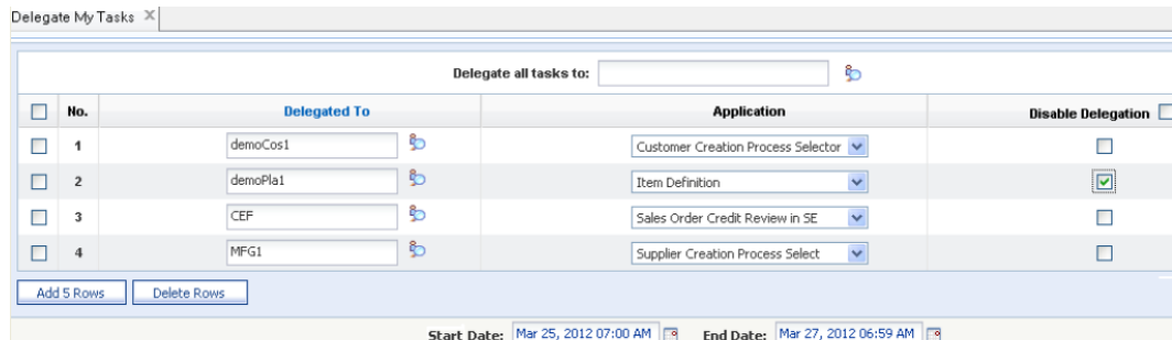
Fig. 2.31 Delegate Applications
