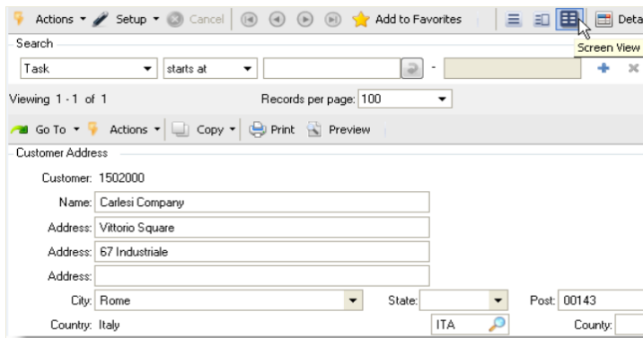
Fig. 2.7 Screen View
