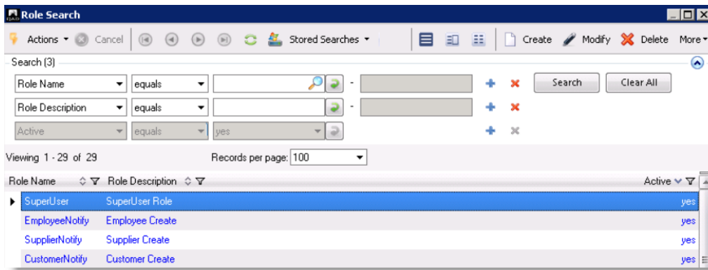
Fig. 2.56 Role Search
