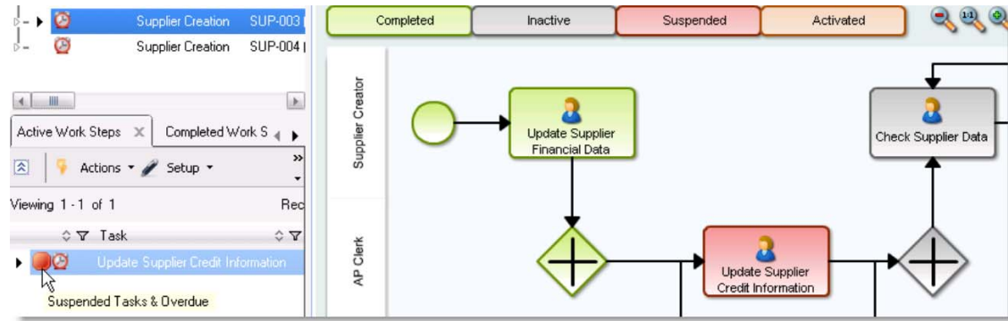
Fig. 2.40 Suspended Task
