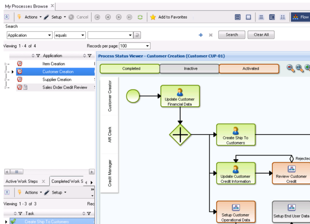
Fig. 2.33 Flow View
