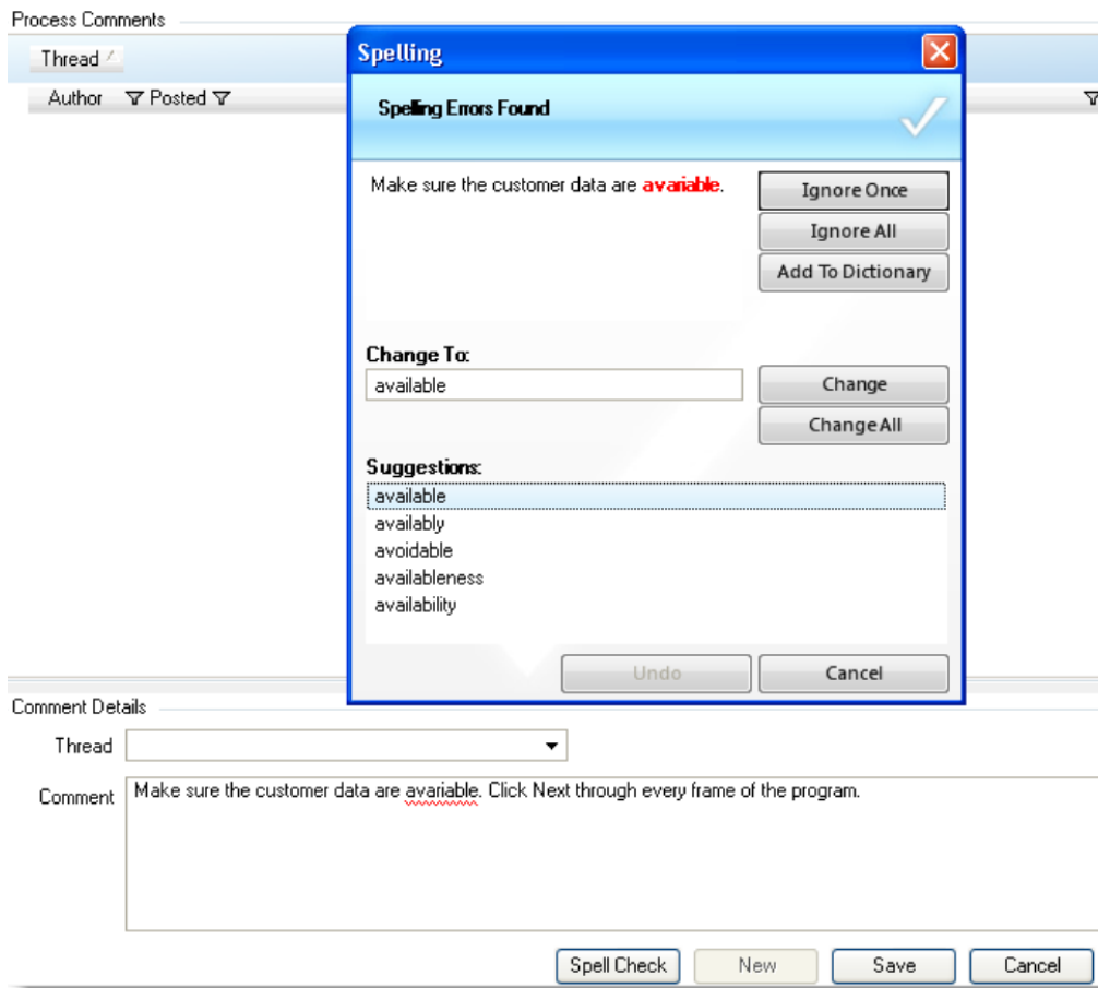
Fig. 2.52 Add Comments
