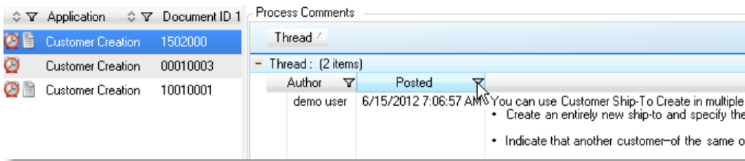
Fig. 2.54 Filter Comments
