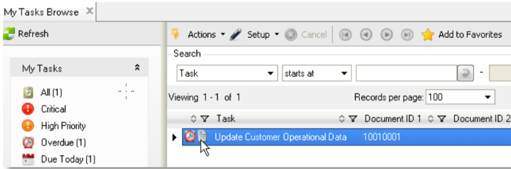
Fig. 2.53 View Comments
