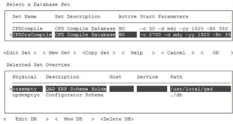
Fig. 2.22 Configure Database Set
