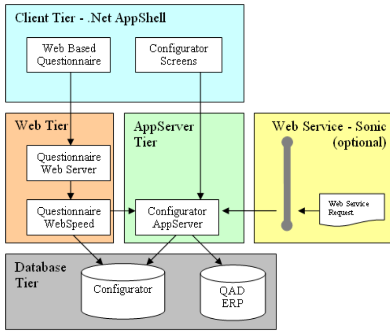
Fig. 1.2 QAD Configurator Deployment Architecture
