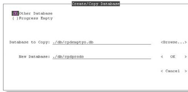
Fig. 1.17 Create Configurator Oracle Production Database
