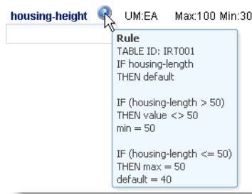
Fig. 7.15 Question Help
