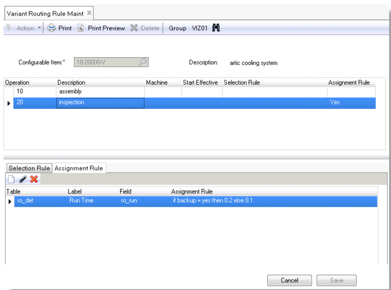
Fig. 6.10 Variant Routing Rule Maintenance
