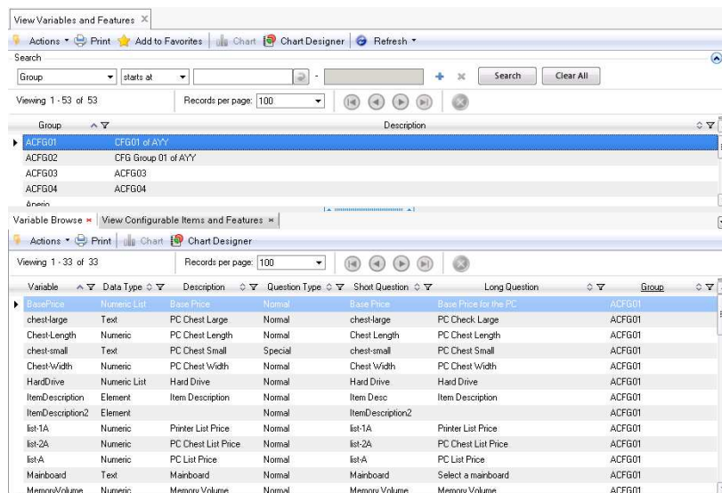
Fig. 3.7 View Variables and Features Browse Collection
