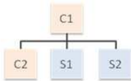
Fig. 8.14 Multi-level Configurations
