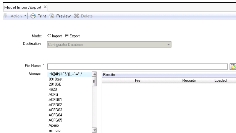
Fig. 8.5 Model Export
