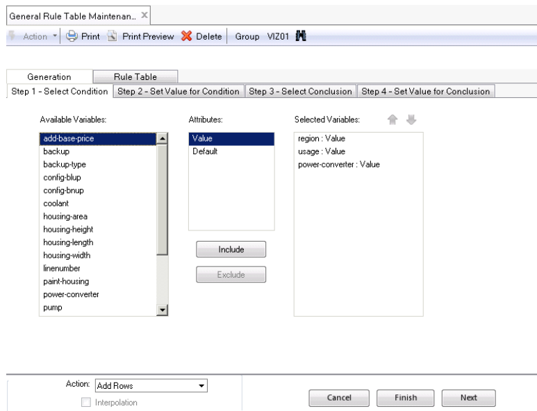
Fig. 5.34 Rule Table Generation - Step 1
