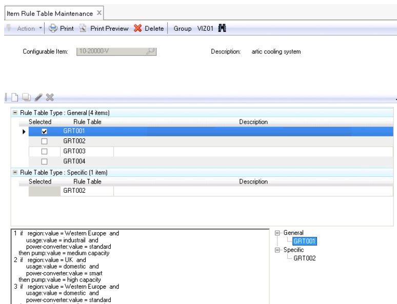
Fig. 5.41 Item Rule Table Maintenance
