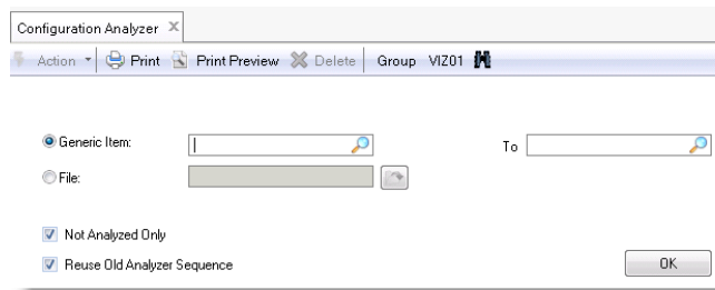
Fig. 5.44 Configuration Analyzer
