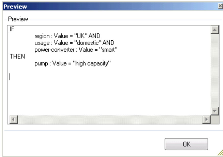
Fig. 5.40 Rule Preview
