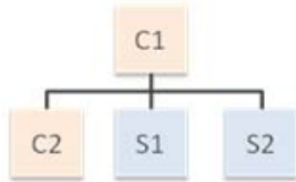
Fig. 8.16 Multi-level Configurations
