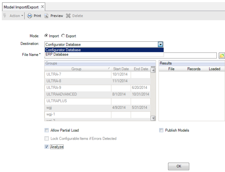
Fig. 8.6 Model Import
