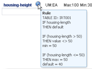
Fig. 7.14 Question Help
