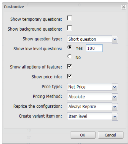
Fig. 7.16 Customize Screen
