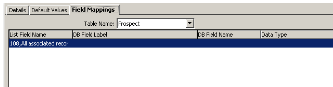
Fig. 14.4 Field Mappings
