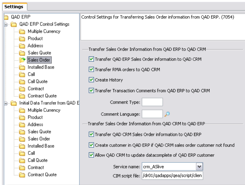
Fig. 12.10 Sales Order
