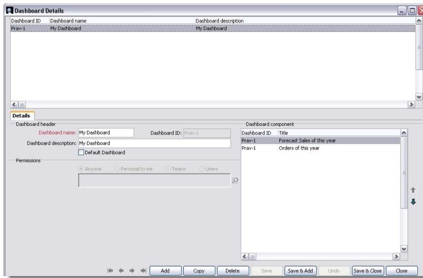
Fig. 12.2 Dashboard Details
