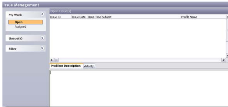
Fig. 16.2 Issue Management
