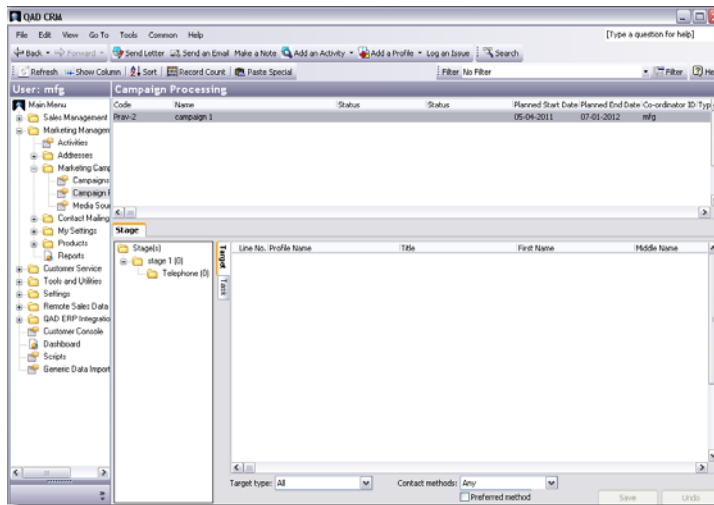
Fig. 14.4 Campaign Processing
