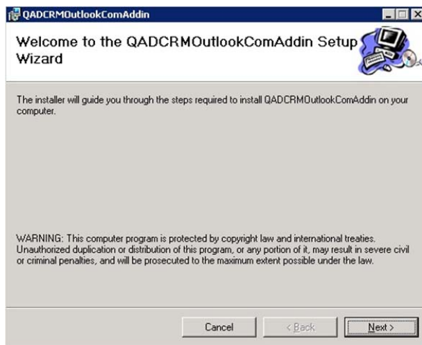
Fig. 1.7 Welcome Screen
