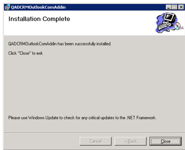
Fig. 1.11 Completion Screen
