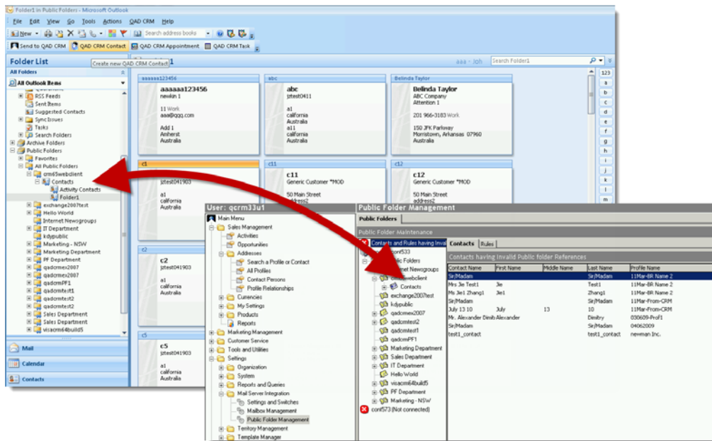
Fig. 1.13 Contact Synchronization
