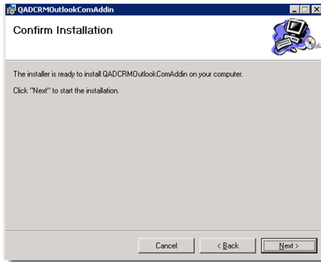
Fig. 1.10 Confirmation Screen
