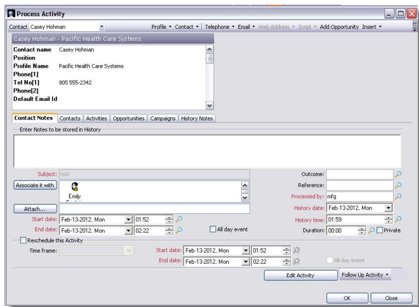
Fig. 5.9 Process Activity
