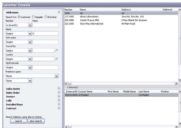
Fig. 9.2 Customer Console
