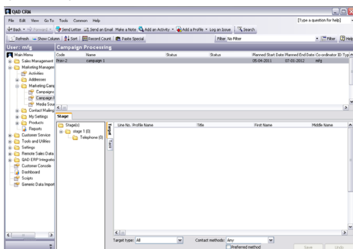
Fig. 15.4 Campaign Processing
