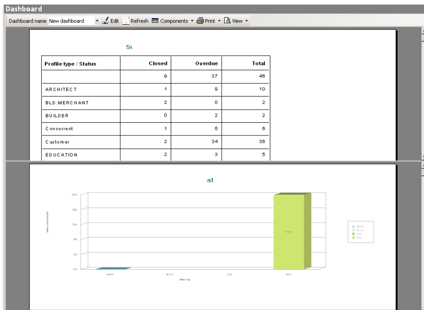
Fig. 13.1 Dashboard
