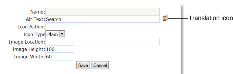
Fig. 1.5 Translation Icon
