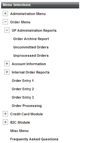
Fig. 3.23 Expandable Menu
