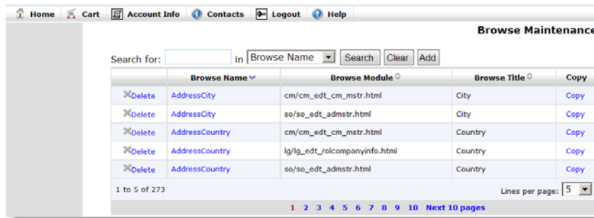
Fig. 3.3 Browse Maintenance
