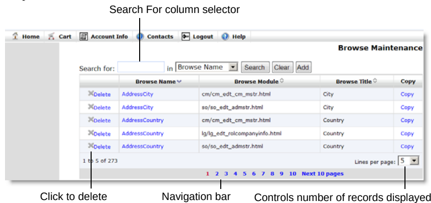
Fig. 1.1 Sample Maintenance Screen
