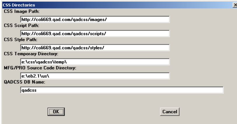
Fig. 3.14 Set Directory Paths Screen
