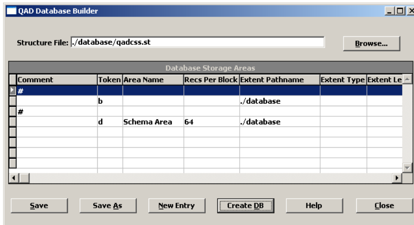
Fig. 2.3 qadcass Structure File
