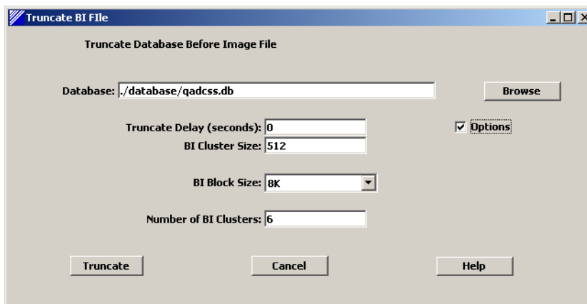
Fig. 2.8 qadcss Truncate BI File Screen
