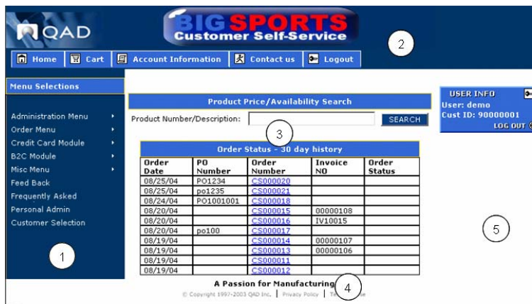
Fig. 5.7 Home Page Functional Areas
