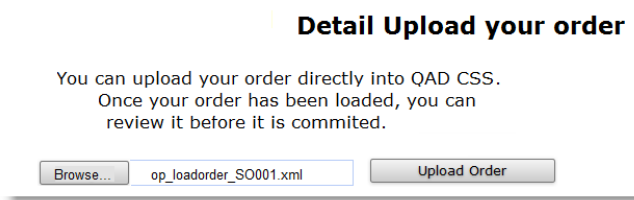
Fig. 5.34 Uploading Order
