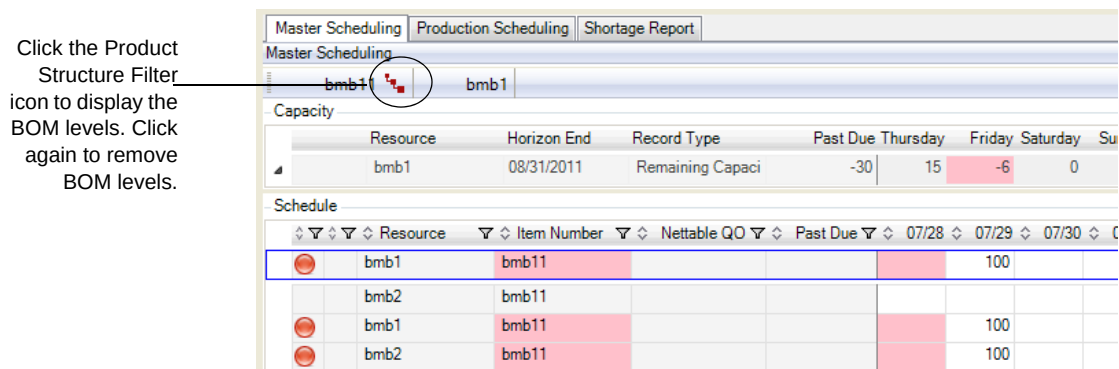
Fig. 9 Schedule Grid Product Structure Filter
