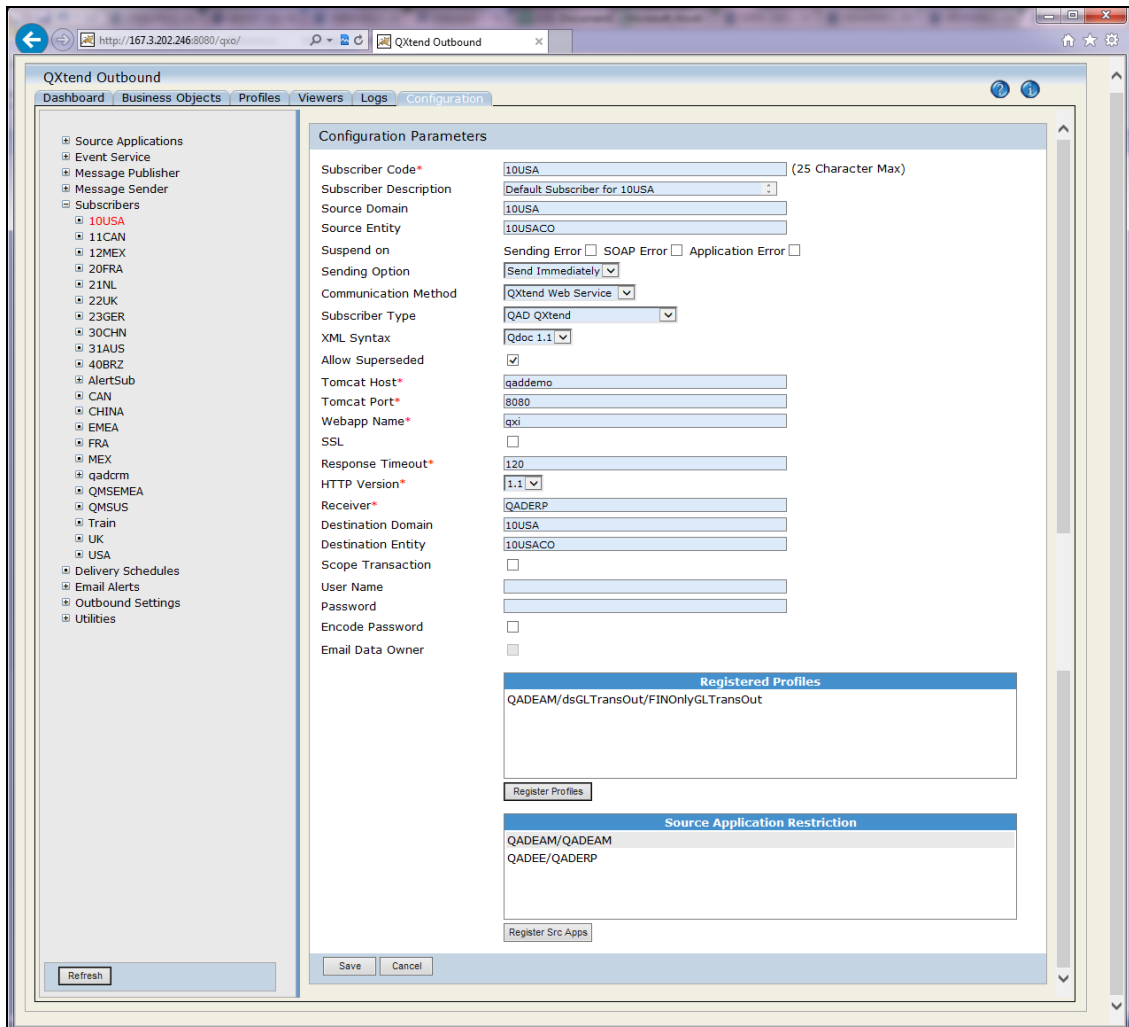
Fig. 6.23. QXO Subscriber
