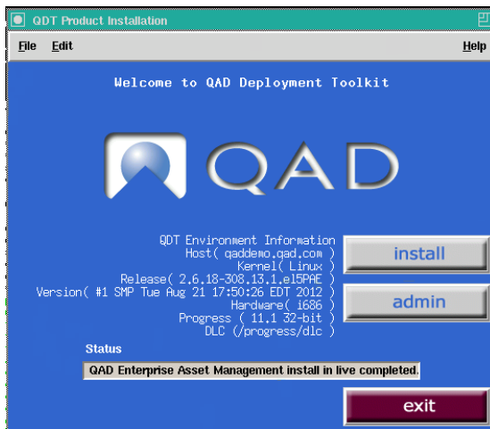
Fig. 3.1 Select Admin
