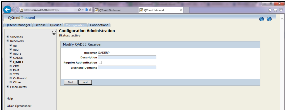
Fig. 6.26. QXI Receiver
