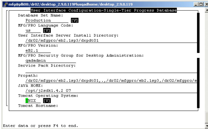
Fig. 4.4 First Single-Tier Configuration Screen
