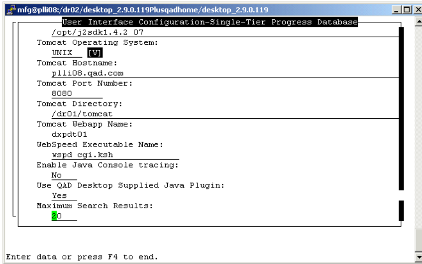
Fig. 4.5 Second Single-Tier Configuration Screen
