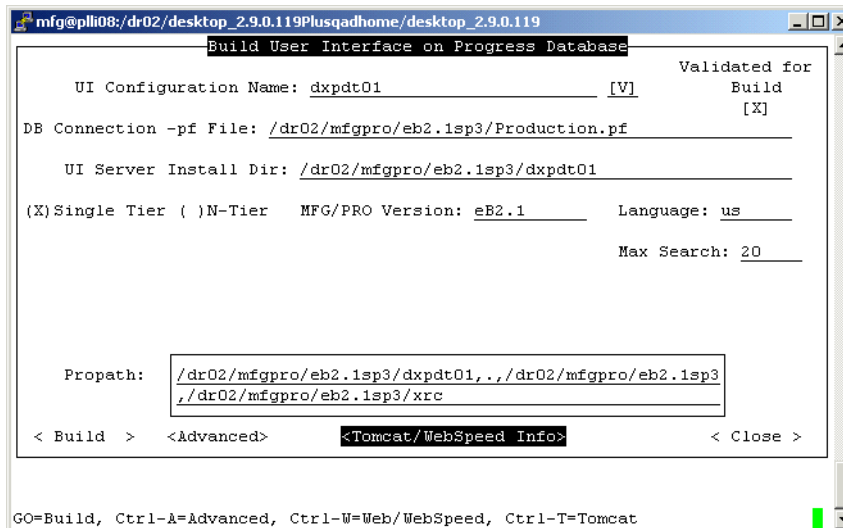
Fig. 4.6 Build User Interface
