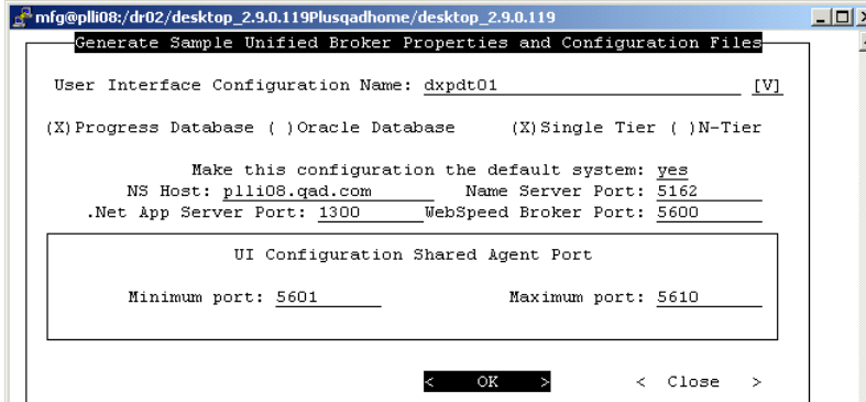
Fig. 4.11 Generate Sample Unified Broker Properties and Configuration Files
