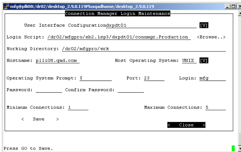
Fig. 4.14 Connection Manager Login Maintenance
