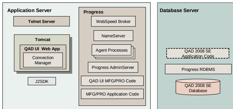
Fig. 1.2 Isolated Database Server Deployment
