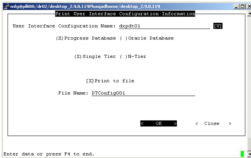
Fig. 4.15 MFG/UTIL Print UI Configuration Information
