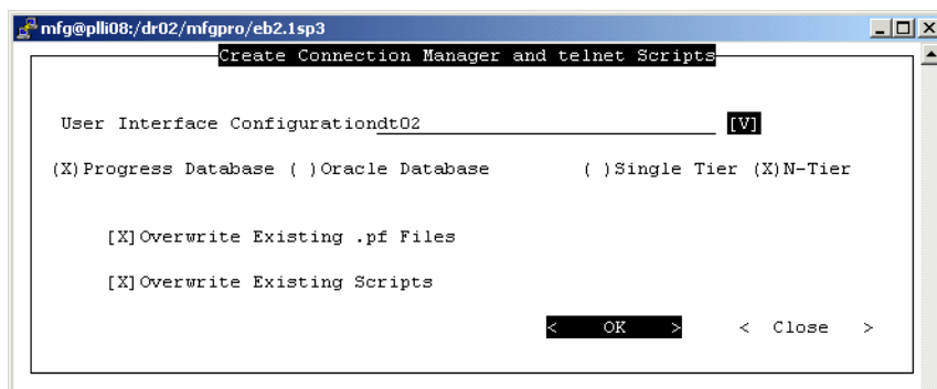
Fig. 5.15 MFG/UTIL Create Connection Manager and telnet Scripts
