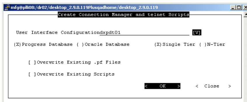
Fig. 4.13 MFG/UTIL Create Connection Manager and telnet Scripts
