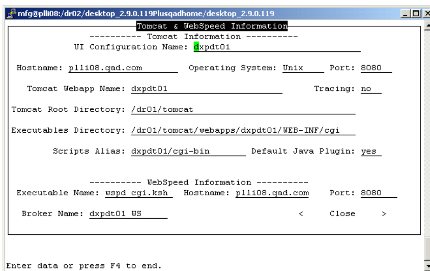
Fig. 4.7 Tomcat Server and WebSpeed Information
