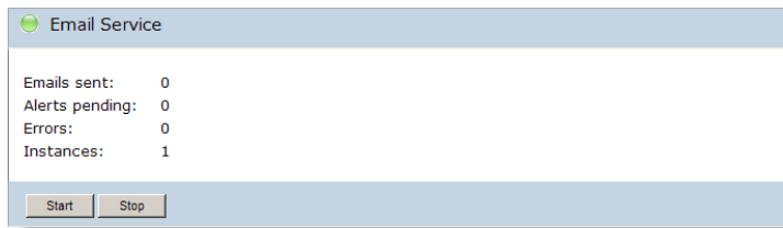
Fig. 2.40 Email Service
