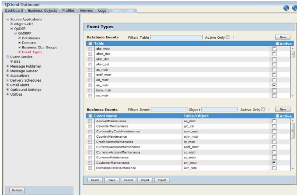
Fig. 2.9 Event Types
