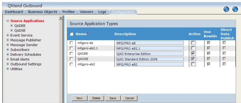
Fig. 2.1 Creating a New Source Application Type
