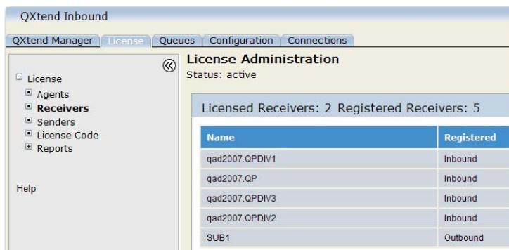
Fig. 22.8 Licensed Receivers
