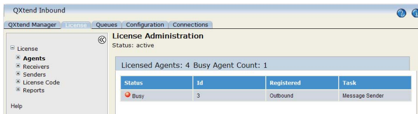
Fig. 22.7 Licensed Agents
