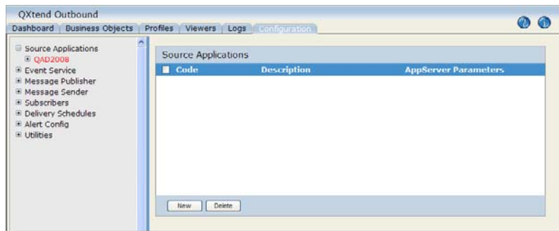
Fig. 2.2 Source Applications
