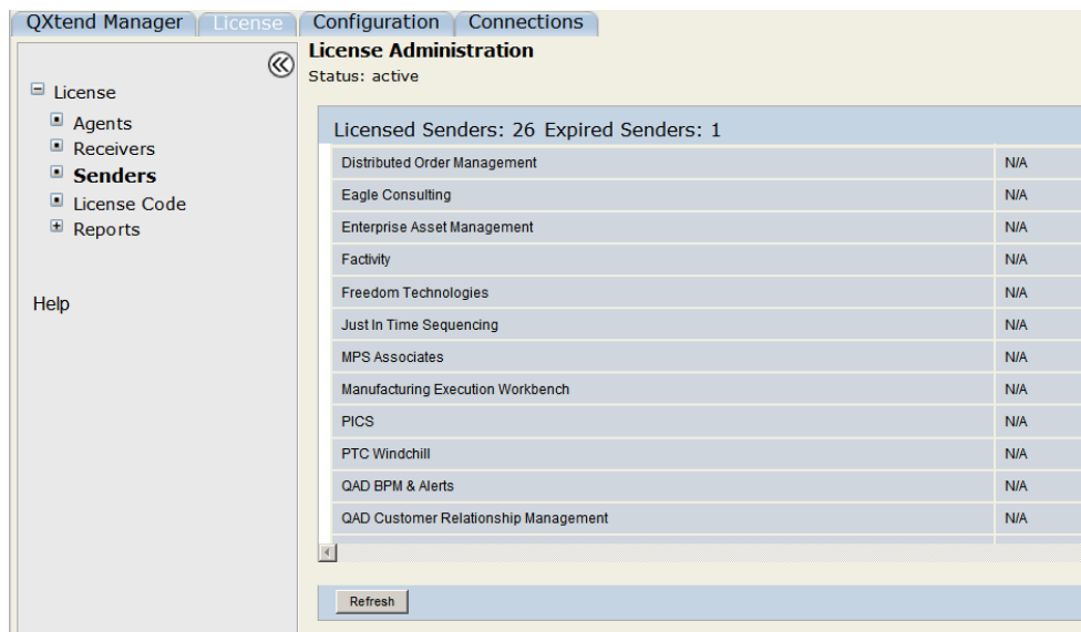
Fig. 22.9 Licensed Senders
