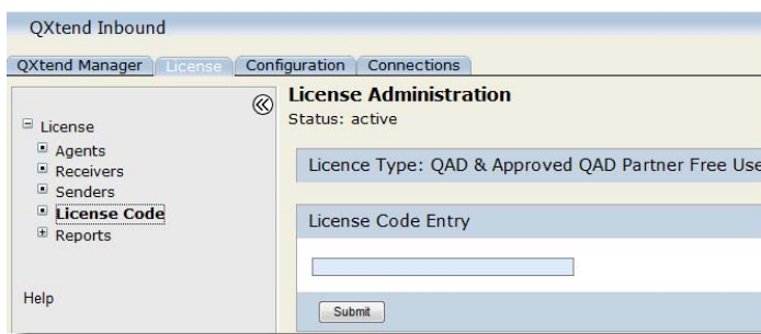
Fig. 22.6 License Administration
