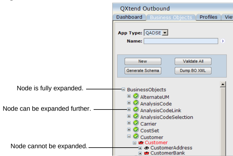
Fig. 1.4 Navigation Tree
