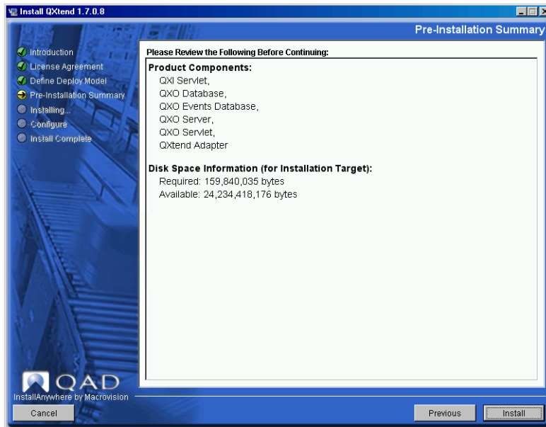
Fig. 4.14 Pre-installation Summary
