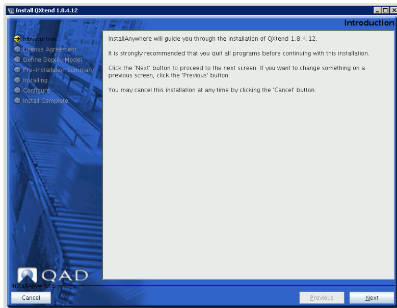
Fig. 4.3 Introduction Screen
