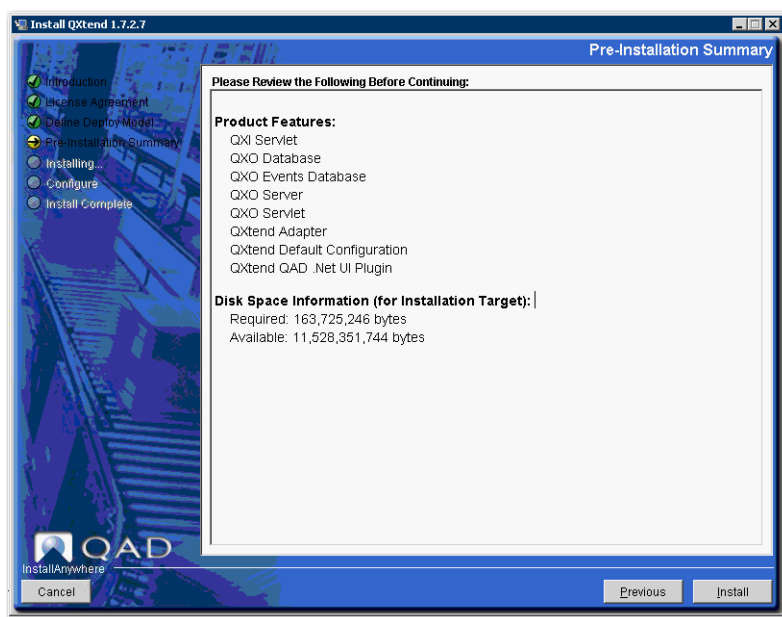
Fig. 4.15 Pre-installation Summary
