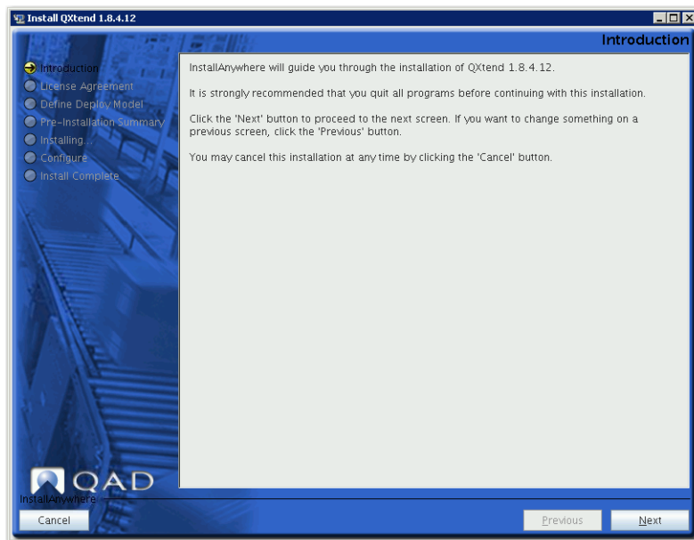
Fig. 4.3 Introduction Screen
