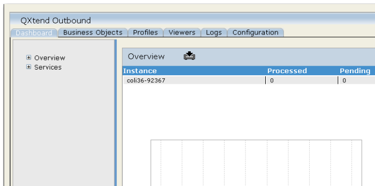
Fig. 7.2 QXO Dashboard
