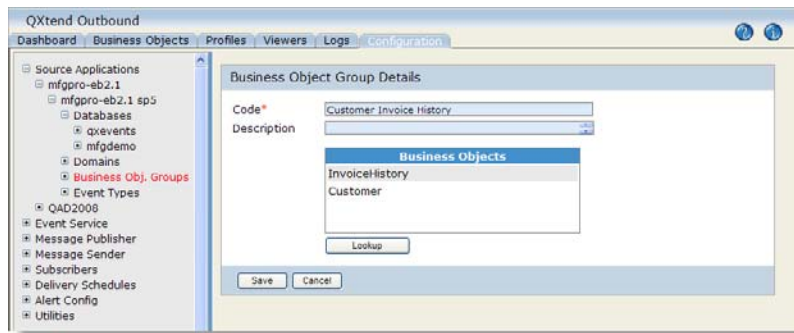
Fig. 2.7 Business Object Group Details
