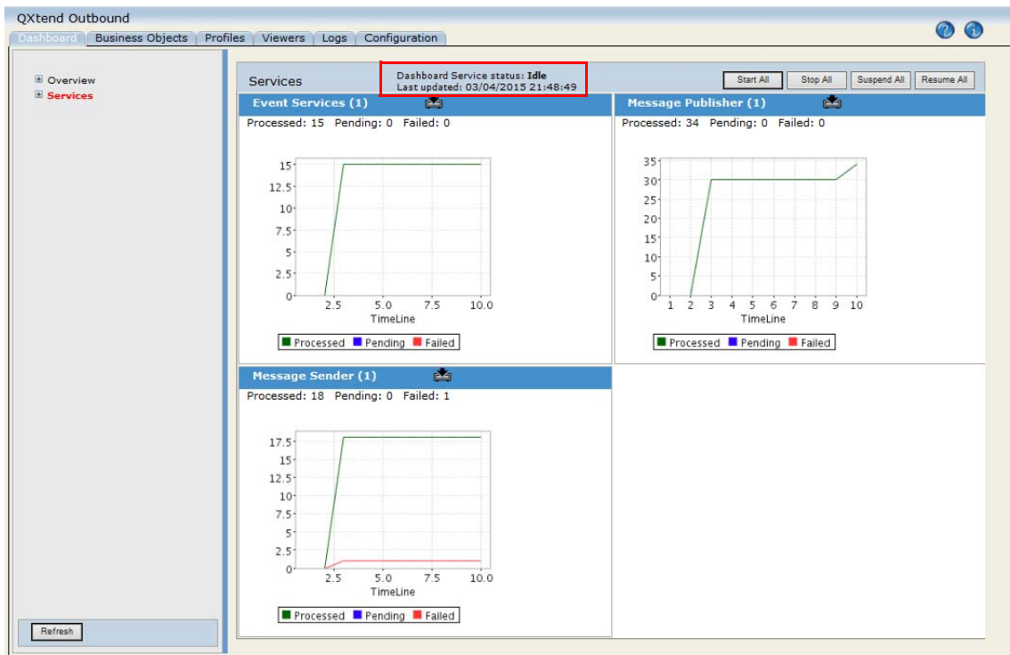
Fig. 5.9 Dashboard Service Status Display
