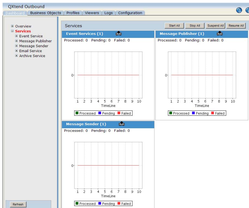
Fig. 11.14 Services
