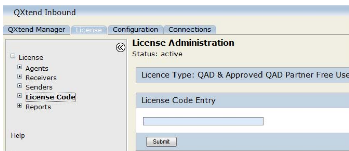
Fig. 22.6 License Administration
