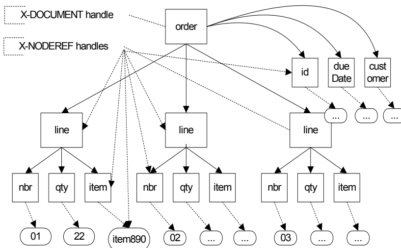
Fig. 28.1 XML Document and DOM Representation
