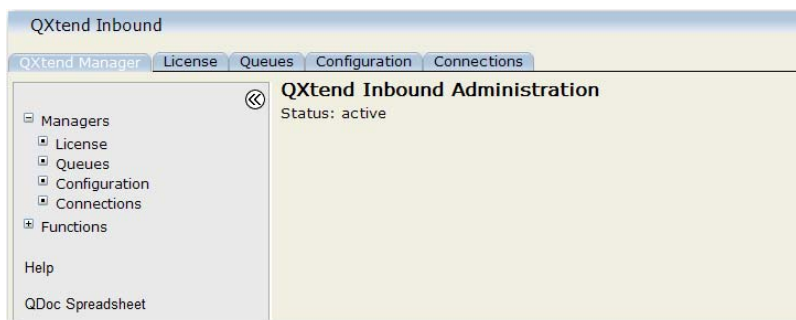
Fig. 14.1 QXtend Manager
