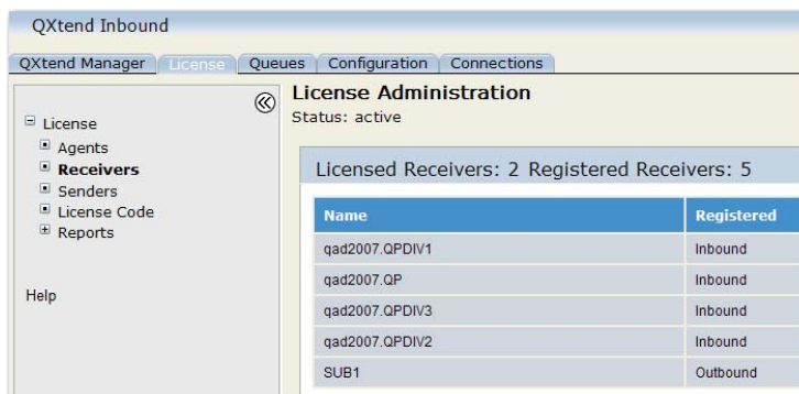
Fig. 22.8 Licensed Receivers
