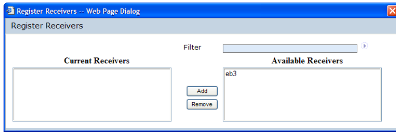
Fig. 16.30 Register Receivers
