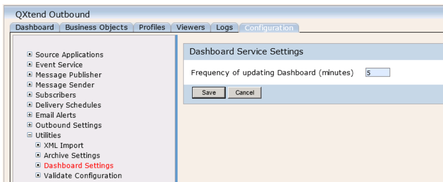
Fig. 5.8 Dashboard Settings
