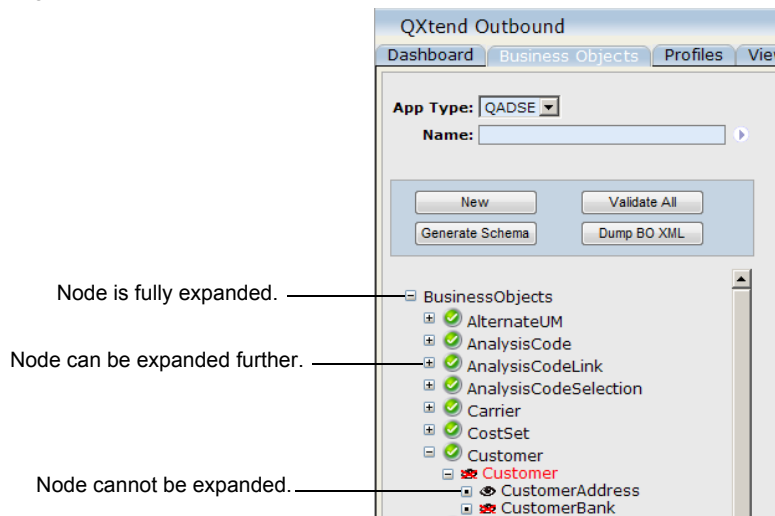
Fig. 1.4 Navigation Tree
