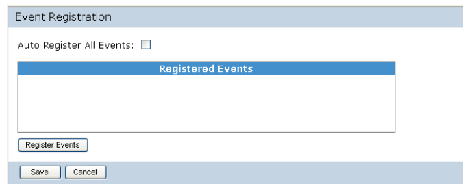
Fig. 2.18 Event Registration
