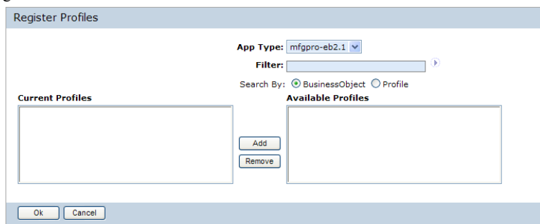
Fig. 2.39 Register Profiles
