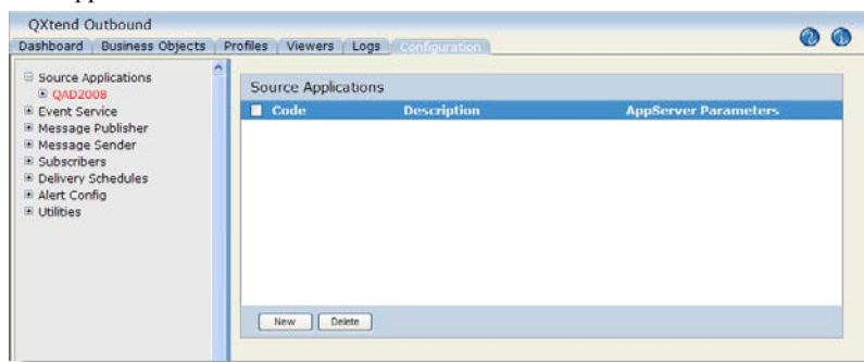
Fig. 2.2 Source Applications
