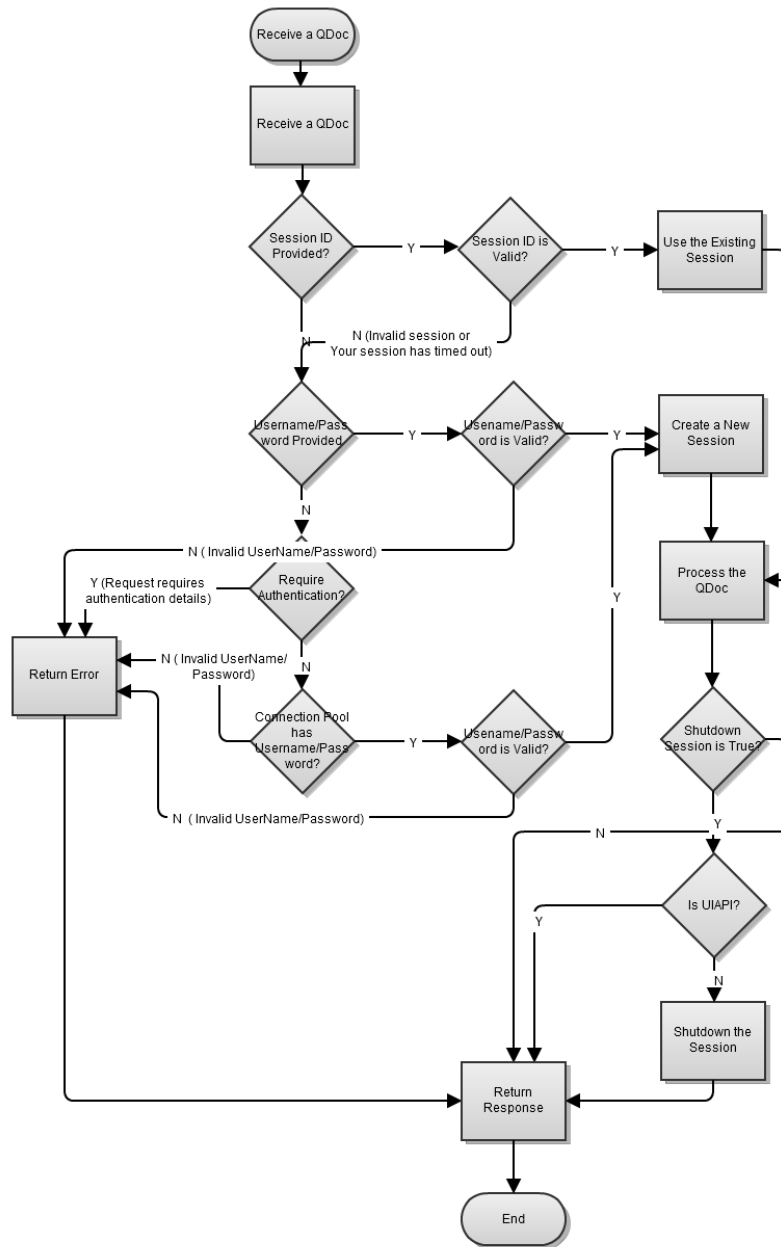
Fig. 13.3 QDoc Authentication
