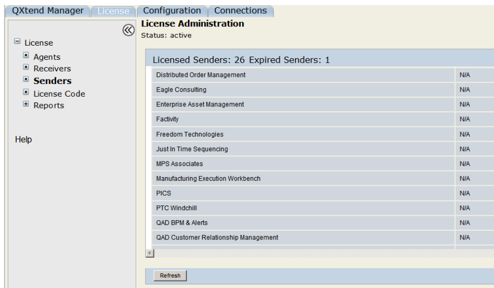
Fig. 22.9 Licensed Senders
