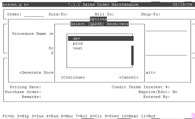
Fig. 18.15 Select Receivers
