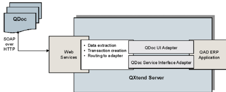
Fig. 13.2 Server Internals
