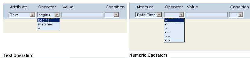
Fig. 6.2 Text Operators
