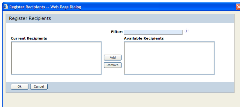
Fig. 2.41 Register Recipients
