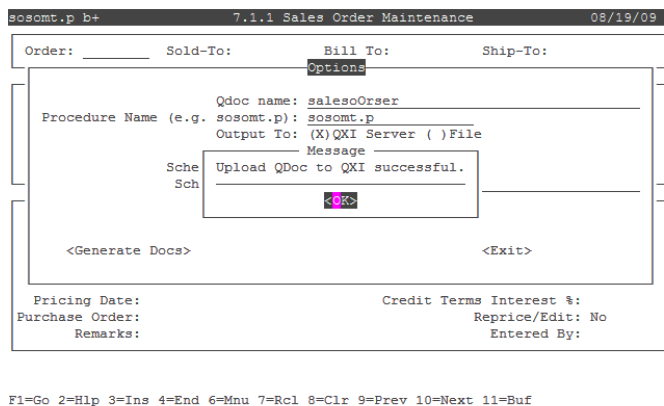
Fig. 18.16 Upload Successful
