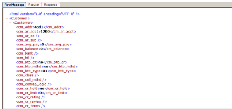
Fig. 9.6 Subscriber Message Details
