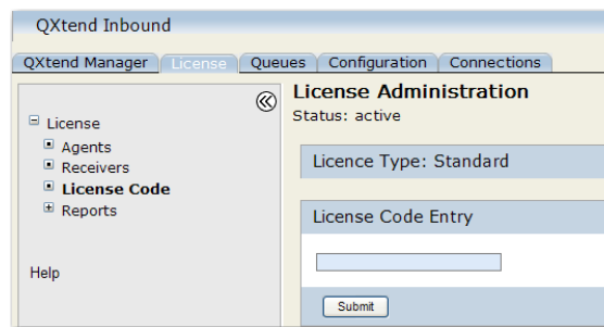
Fig. 22.6 License Administration
