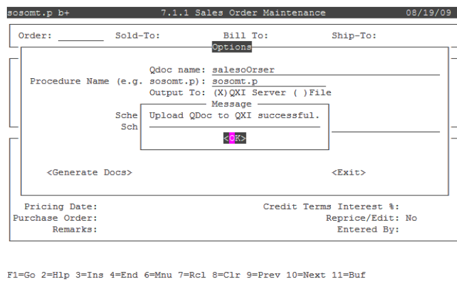
Fig. 18.16 Upload Successful
