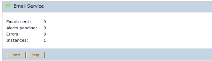
Fig. 2.46 Email Service
