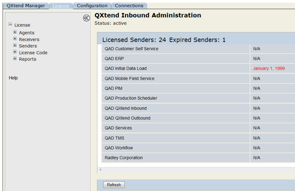
Fig. 22.9 Licensed Senders
