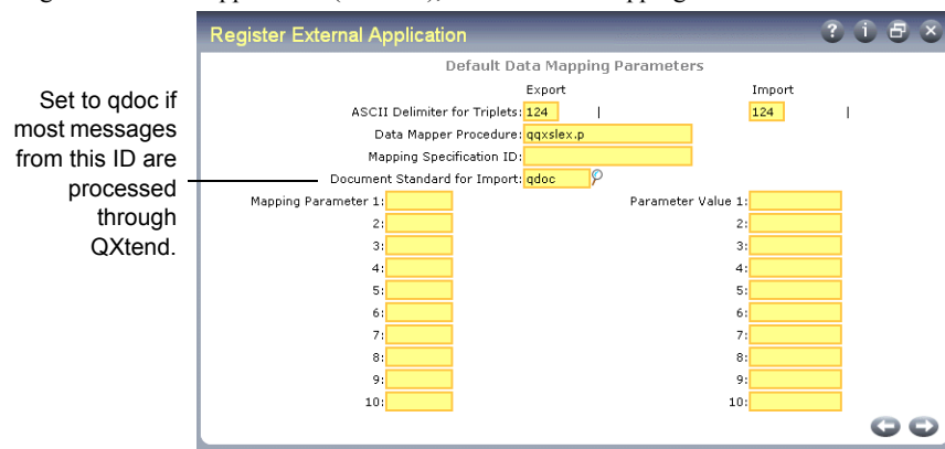
Fig. 21.2 Register External Application (36.8.1.1), Default Data Mapping Parameters
