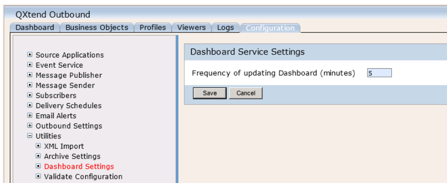
Fig. 5.8 Dashboard Settings
