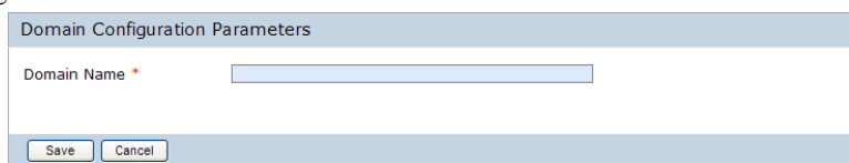
Fig. 16.31 Register Domains
