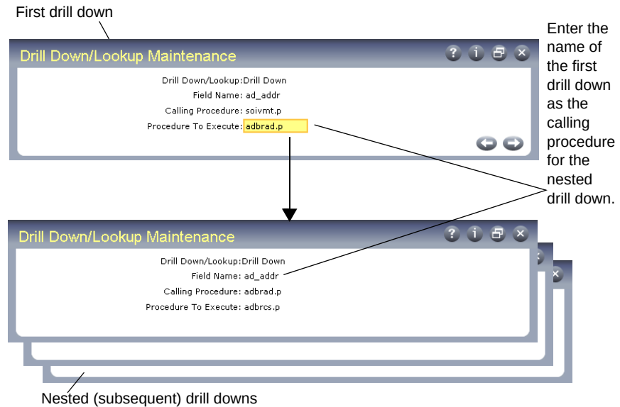
Fig. 11.3 Nested Drill Downs
