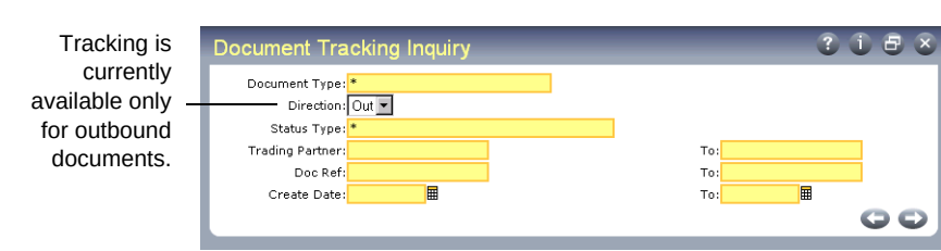
Fig. 6.22 Document Tracking Inquiry (35.9.16.3), First Frame
