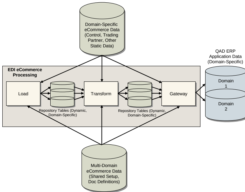
Fig. 5.49 EDI eCommerce Multiple-Domain Processing Flow
