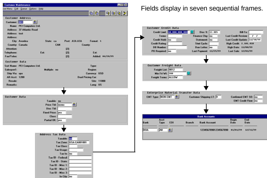
Fig. 1.10 Sample Windows Maintenance Program
