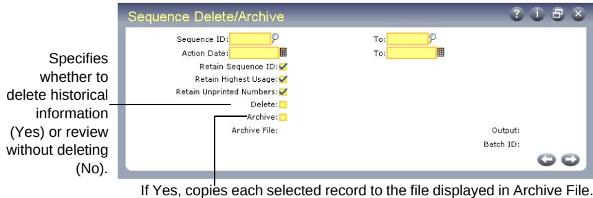
Fig. 2.17 Sequence Delete/ Archive (36.2.21.23)
