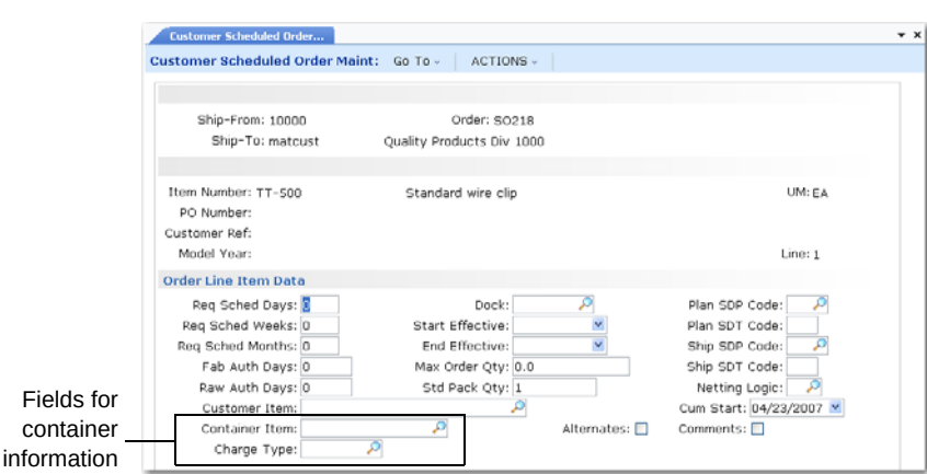
Fig. 4.14 Container Fields in Customer Scheduled Order Maintenance (7.3.13)
