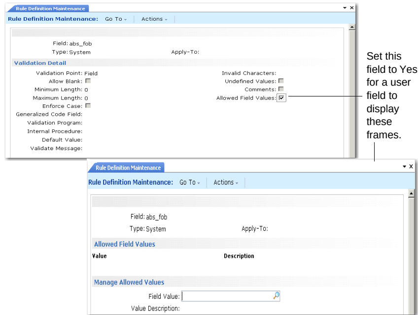
Fig. 6.30 Allowed Field Values and Manage Allowed Values Frames
