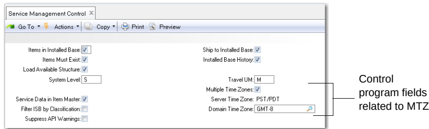
Fig. 4.2 Service Management Control (11.24)
