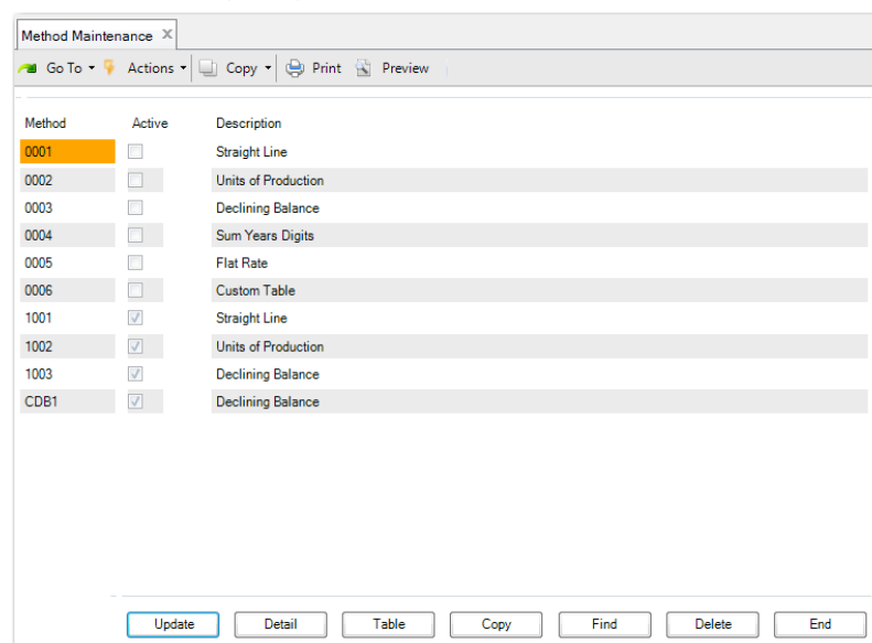
Fig. 2.3 Method Maintenance (32.1.1)
