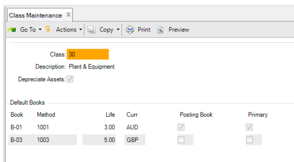
Fig. 2.15 Class Maintenance (32.1.17)
