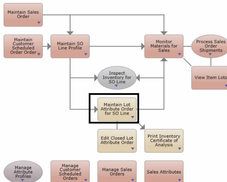
Fig. 3.12 Manage Lot Attribute Order for SO Line Process Map
