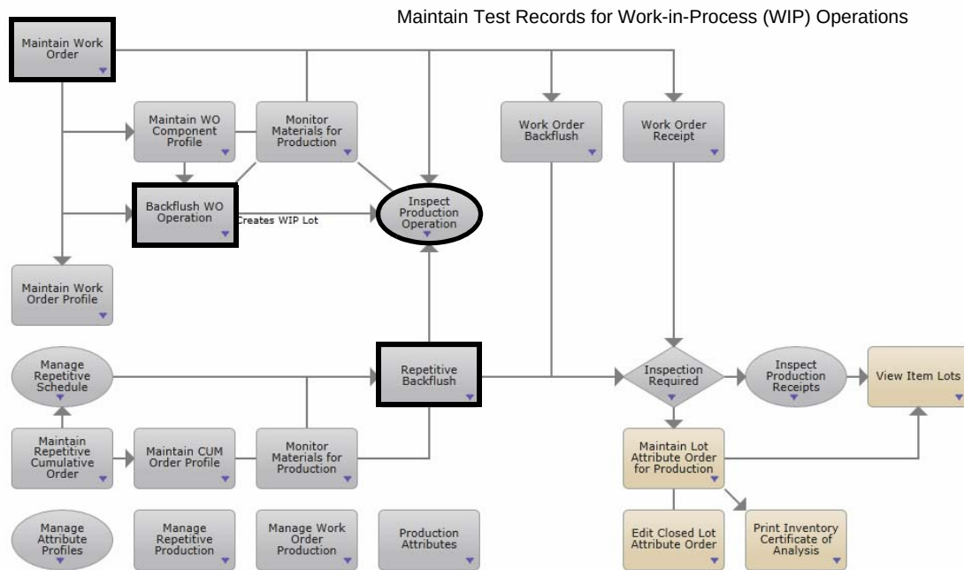
Fig. 4.44 Process Map - Manage Production with Attributes
