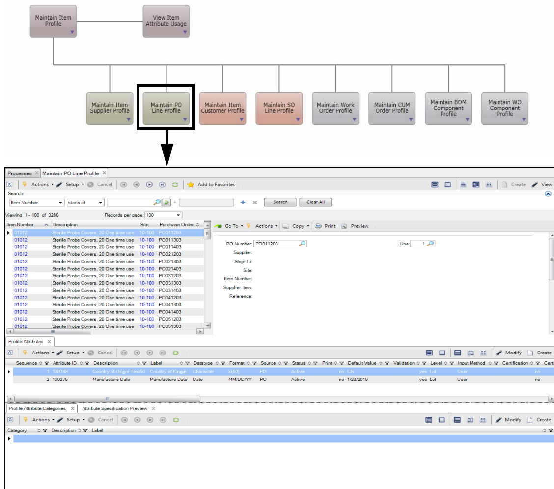
Fig. 3.27 Maintain PO Line Profile
