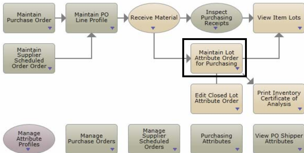
Fig. 3.15 Process Map - Manage Purchasing with Attributes
