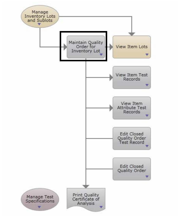
Fig. 4.10 Process Map - Inspect Inventory
