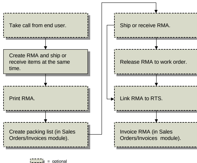
Fig. 23.1 RMA Workflow
