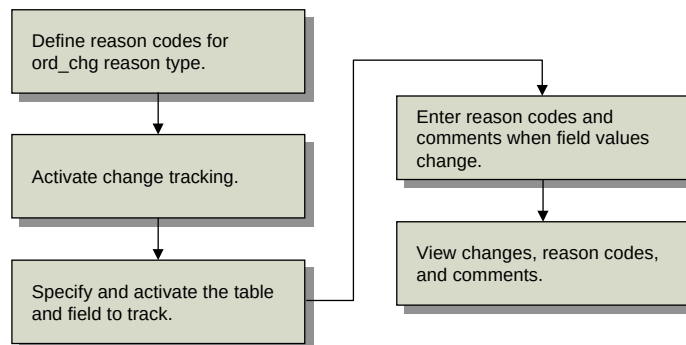
Fig. 2.20 Change Tracking Implementation Flow
