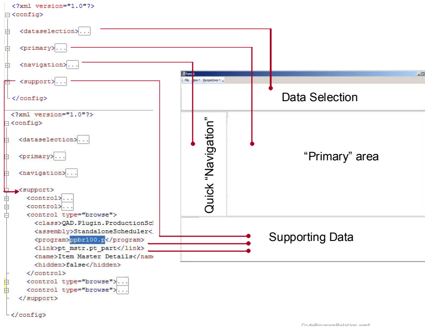
Fig. 4.2 Code-UI Relationship
