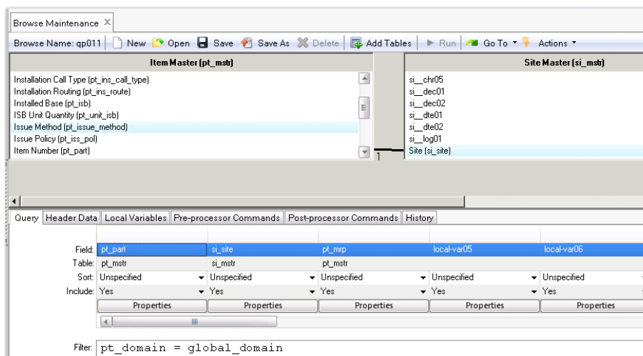
Fig. 4.6 Browse Maintenance (36.20.13)
