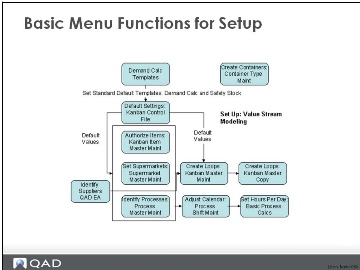
This image shows the basic menu functions involved in setting up data in QAD Lean.
