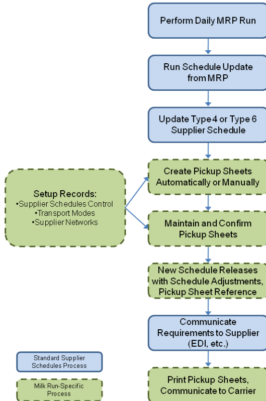
Fig. 6.1 Using Supplier Schedules with Milk Run Pickup Sheets
