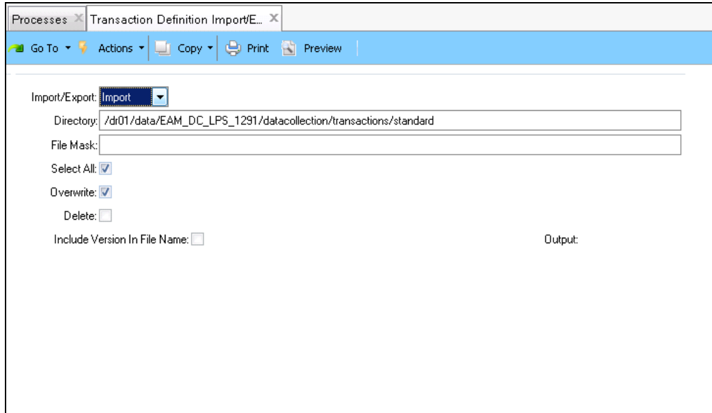
Fig. A.7 Transaction Definition Import/Export
