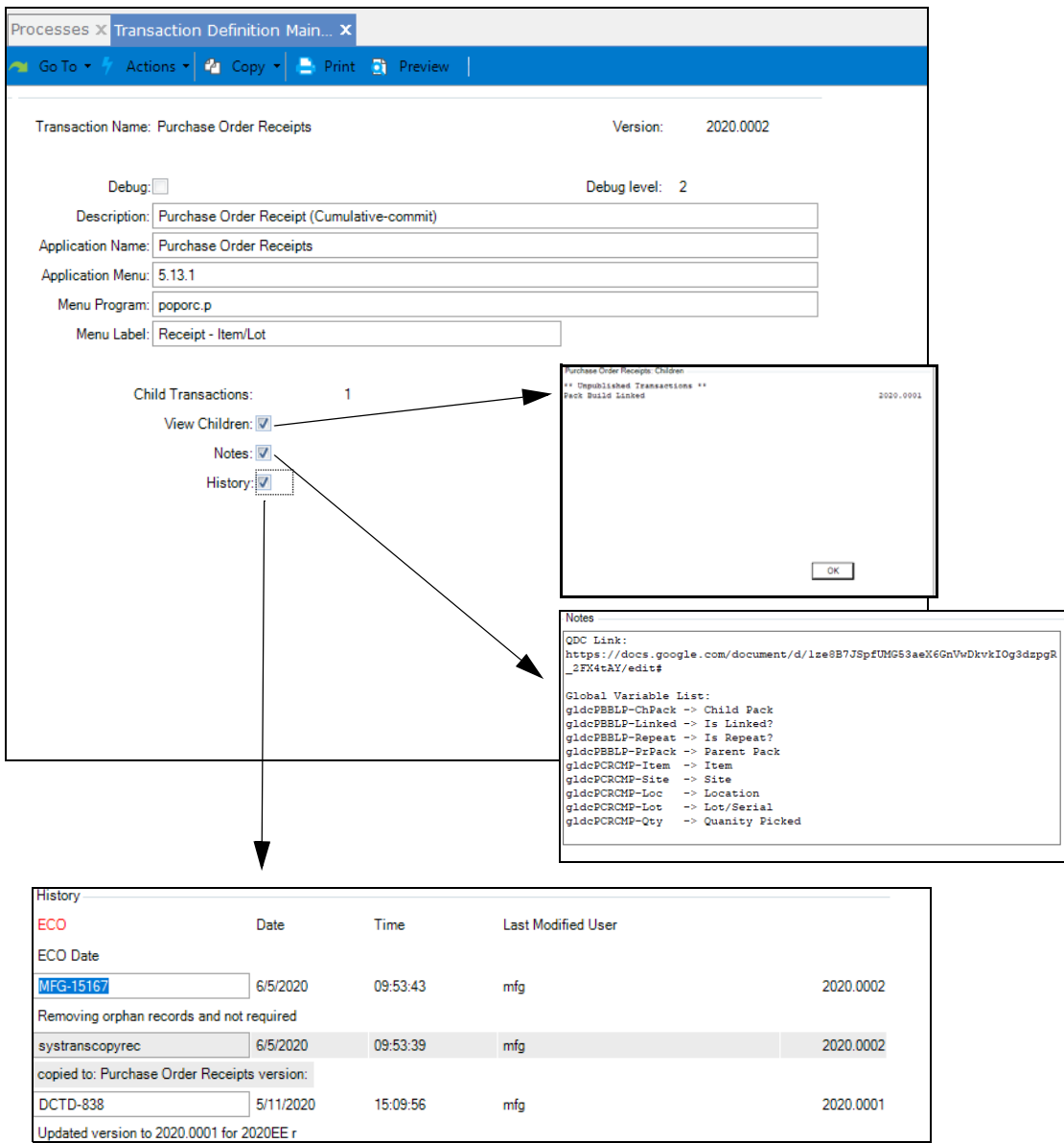
Fig. 3.1 Transaction Definition Maintenance, Header
