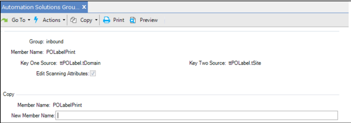
Fig. A.10 Automation Solutions Group Member Maintenance - Clone Member Action
