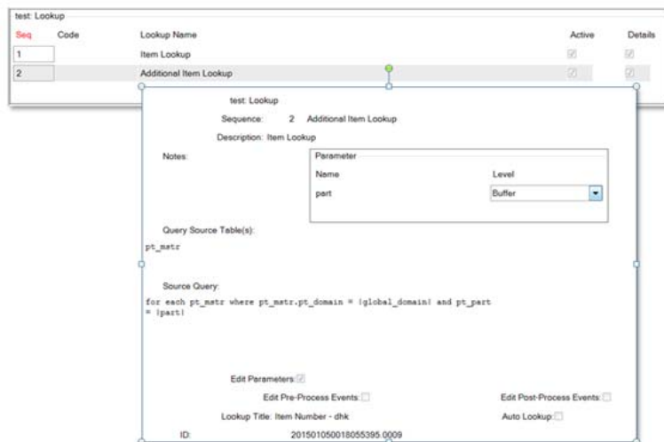
Fig. 3.20 Transaction Definition Maintenance, Drill Down for Lookups
