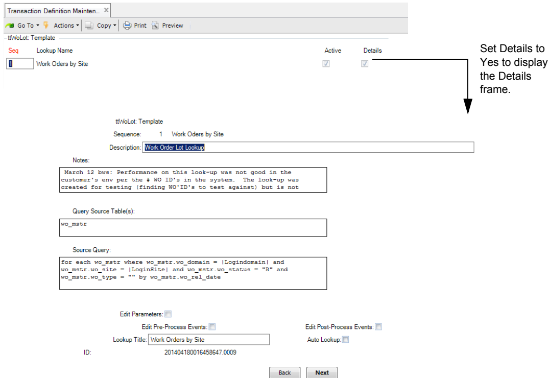
Fig. 3.18 Transaction Definition Maintenance, Lookup Maintenance
